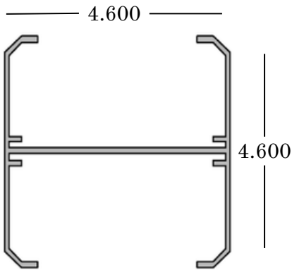
5" Post Stiffener
